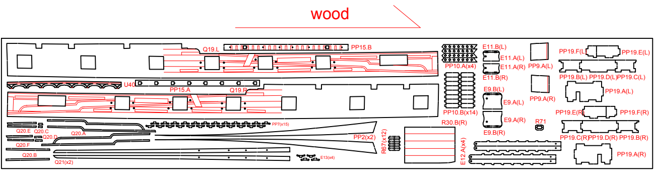
1 mm solid wood - 450 x 90 mm
