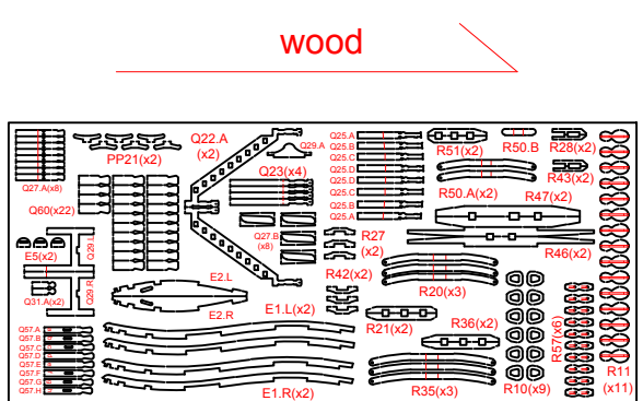
2 mm solid wood - 200 x 90 mm
