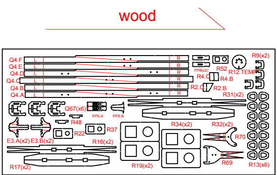
3 mm solid wood - 195 x 90 mm
