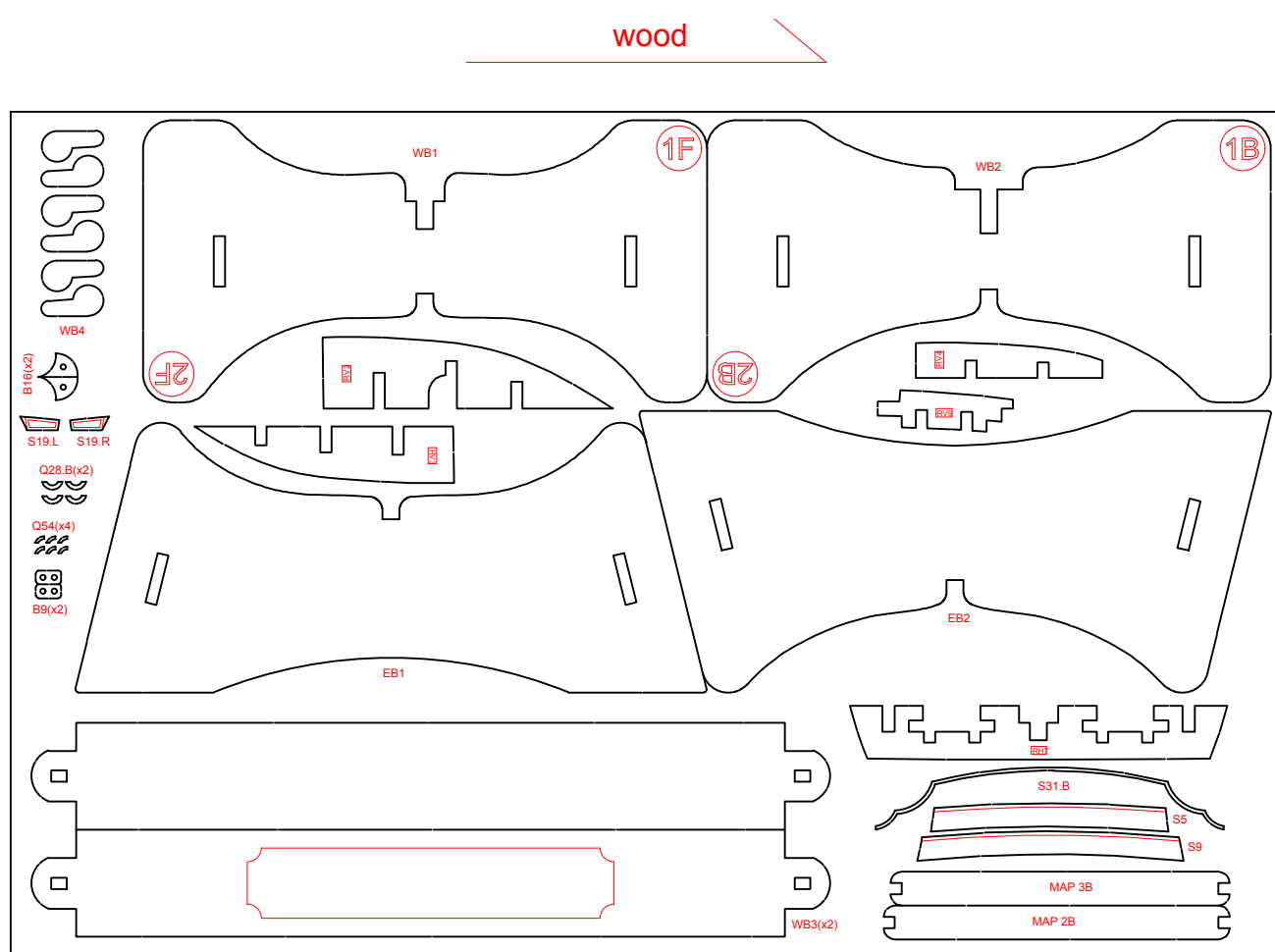
4 mm plywood - 450 x 300 mm
