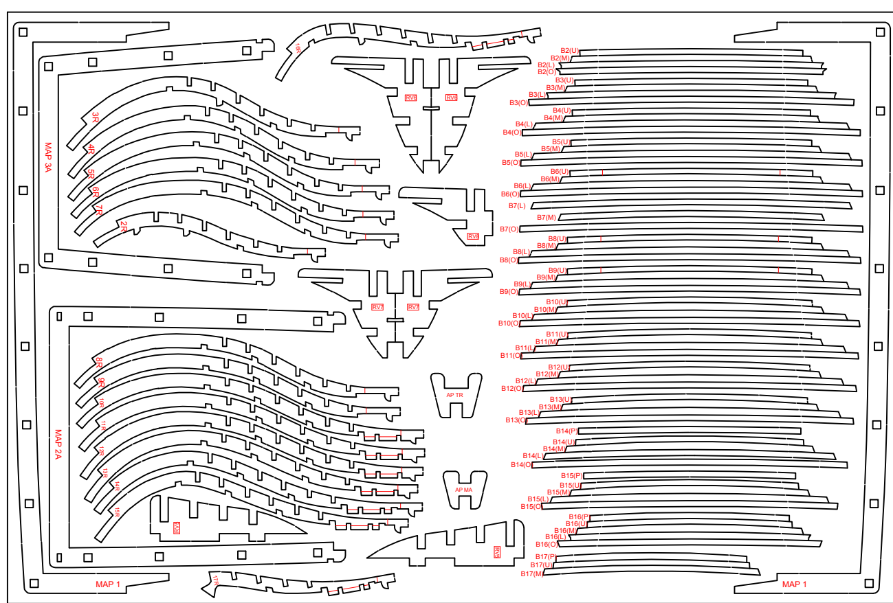
4 mm plywood - 450 x 300 mm
