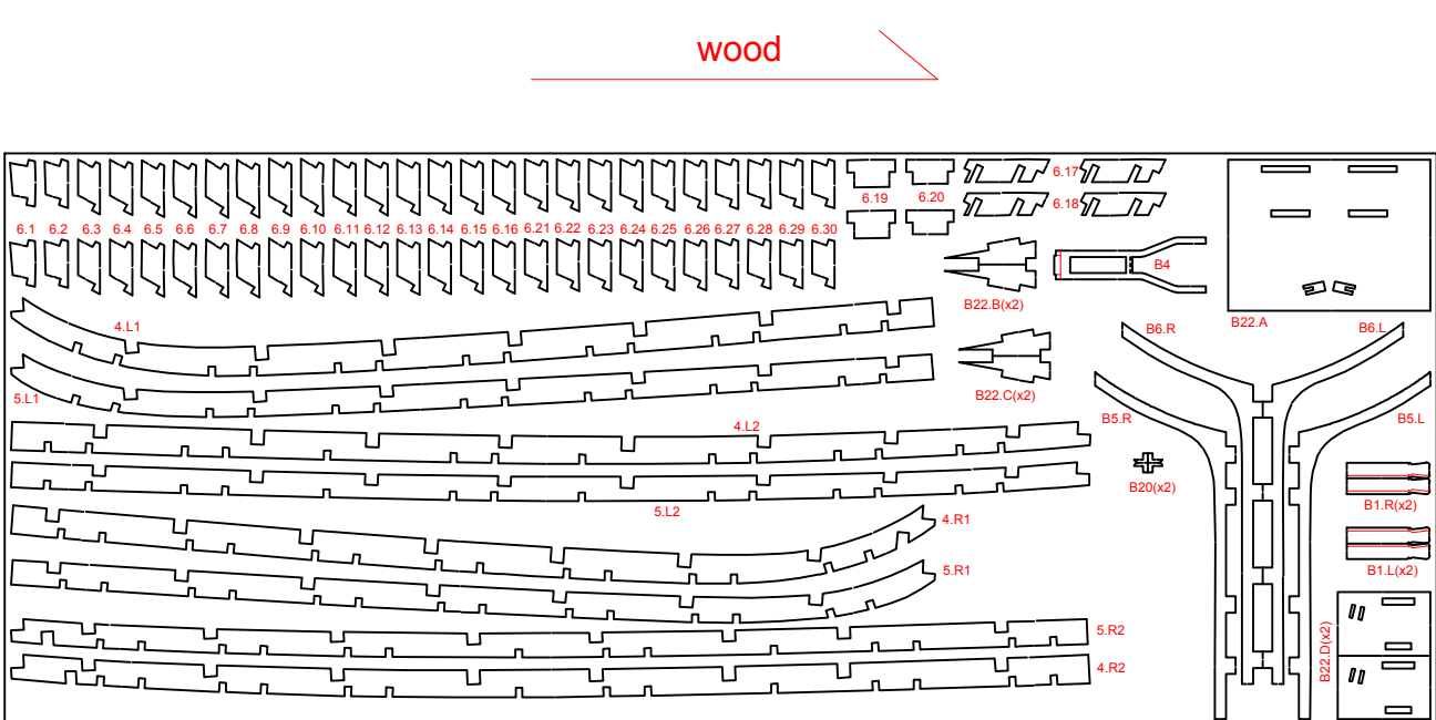
2 mm plywood - 450 x 180 mm
