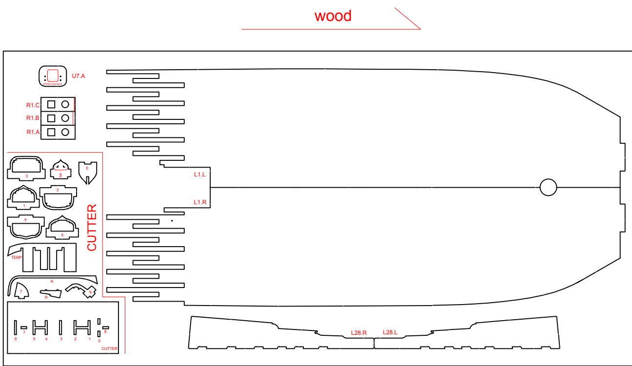
1.5 mm plywood - 450 x 225 mm
