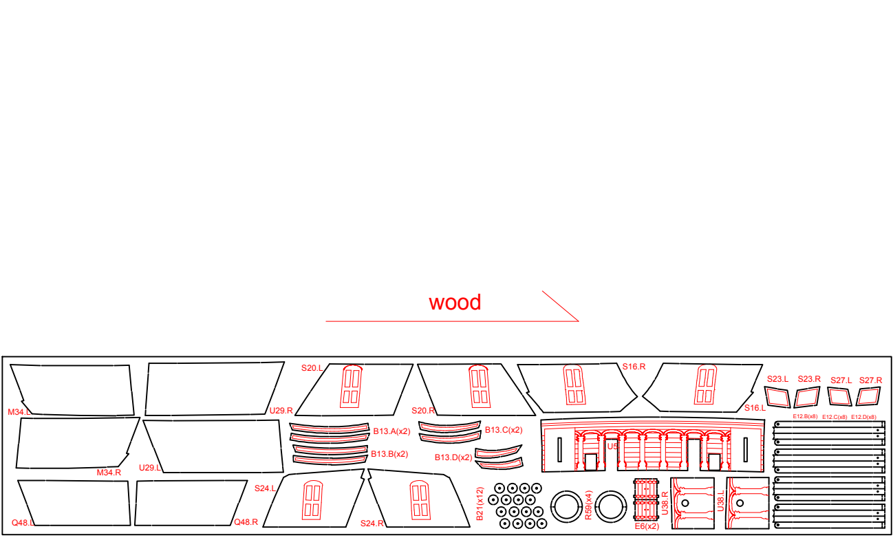
0.5 mm solid wood veneer - 450 x 90 mm
