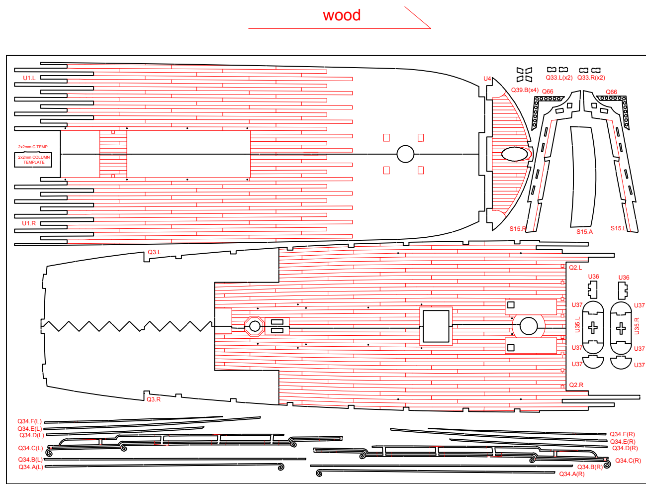
1.5 mm plywood - 450 x 300 mm
