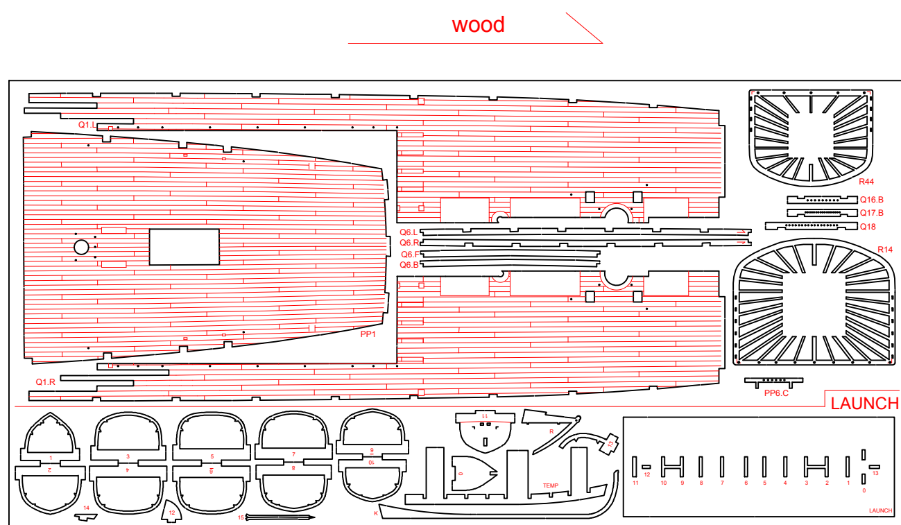
1.5 mm plywood - 450 x 225 mm
