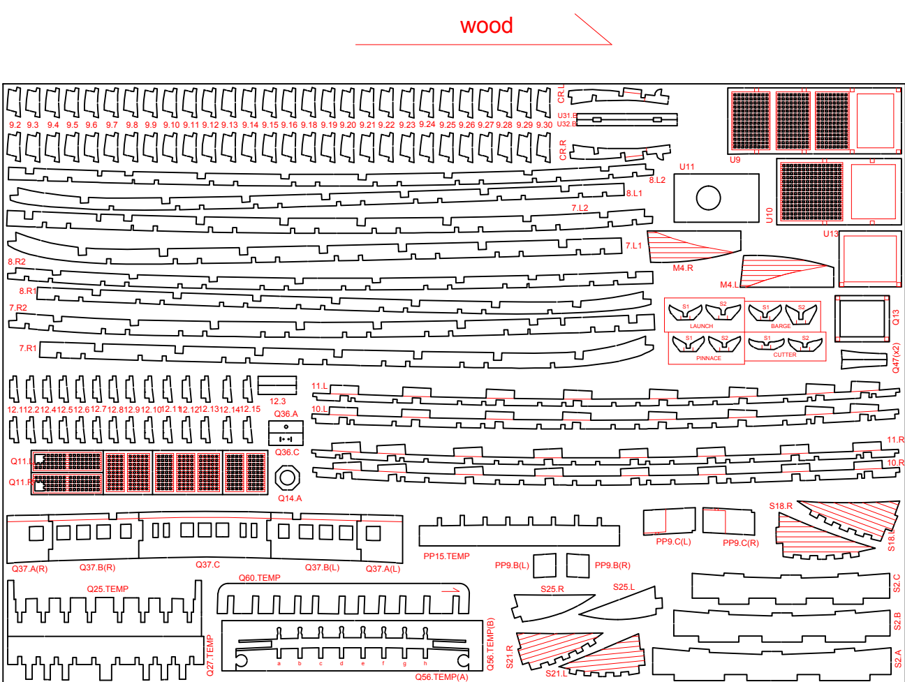
2 mm plywood - 450 x 300 mm
