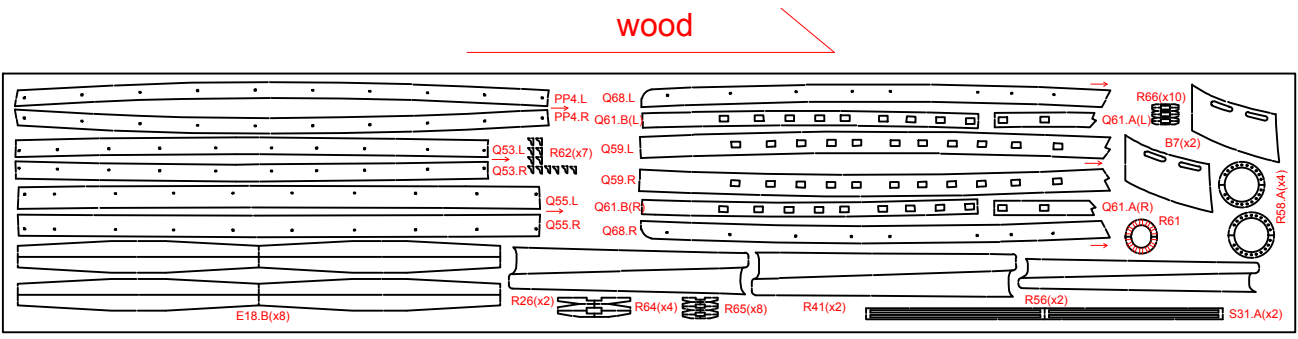
1 mm solid wood - 450 x 90 mm
