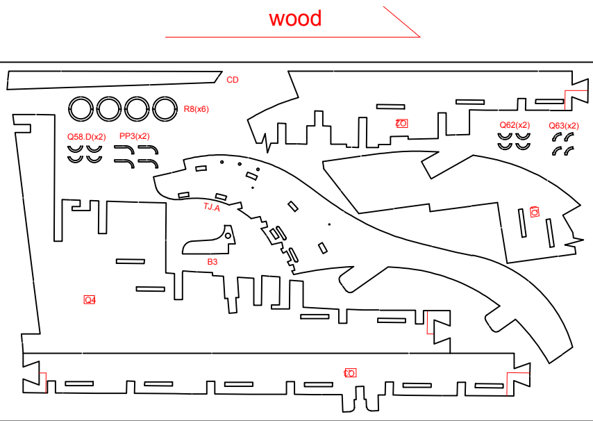
6 mm plywood - 300 x 180 mm
