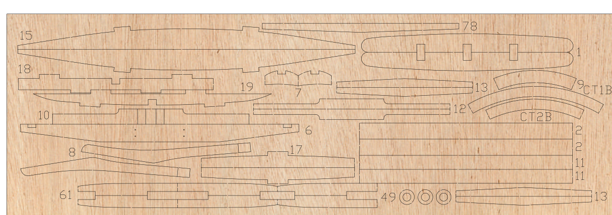
4 mm Plywood - (300 x 100 mm)
