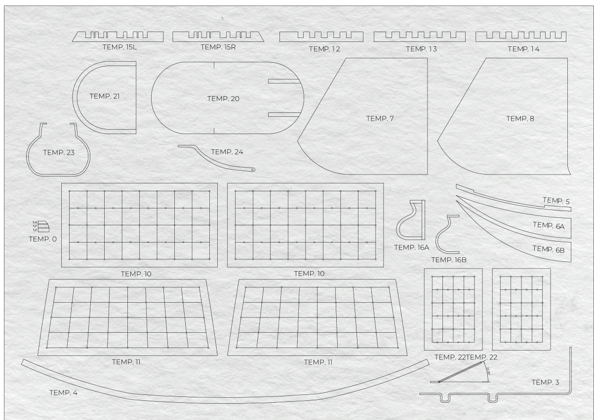
Paper Template 1 - (A4 Size)
