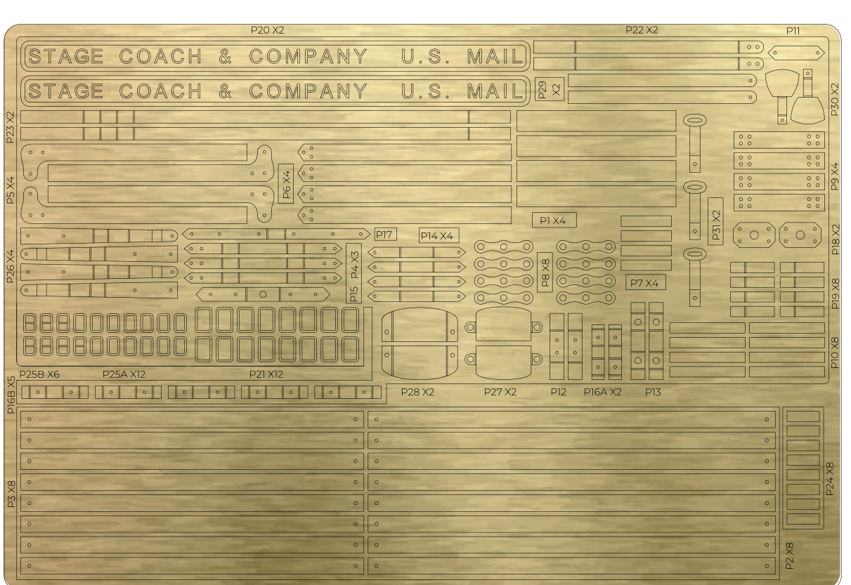
0.3 mm Brass sheet - (200 x 135 mm)
