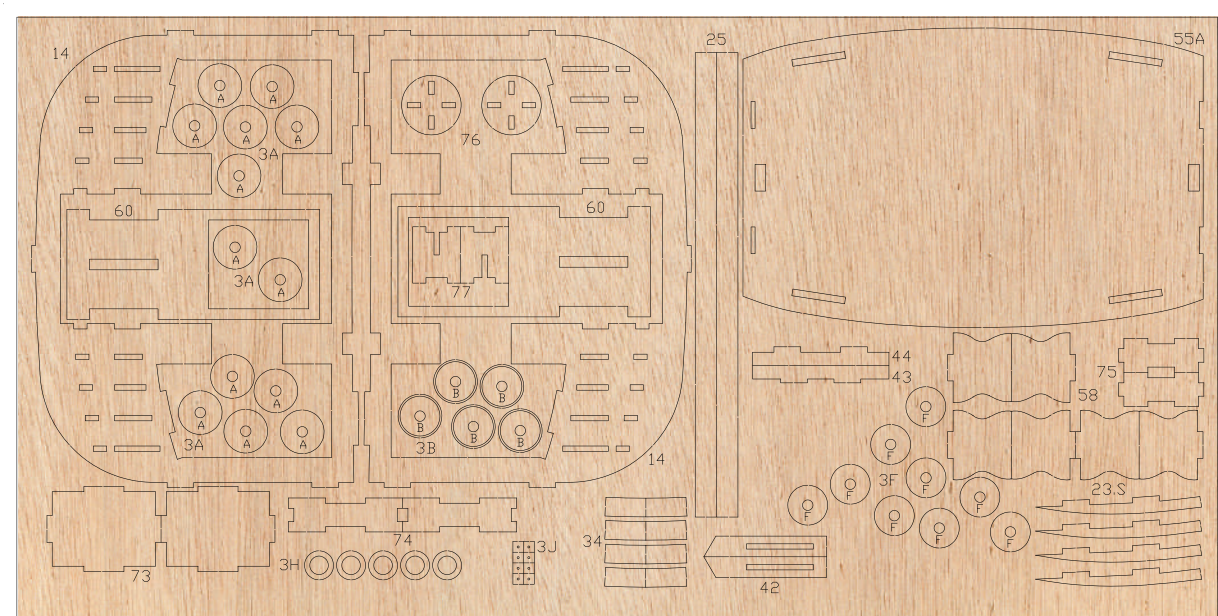
2 mm Plywood - (450 x 225 mm)
