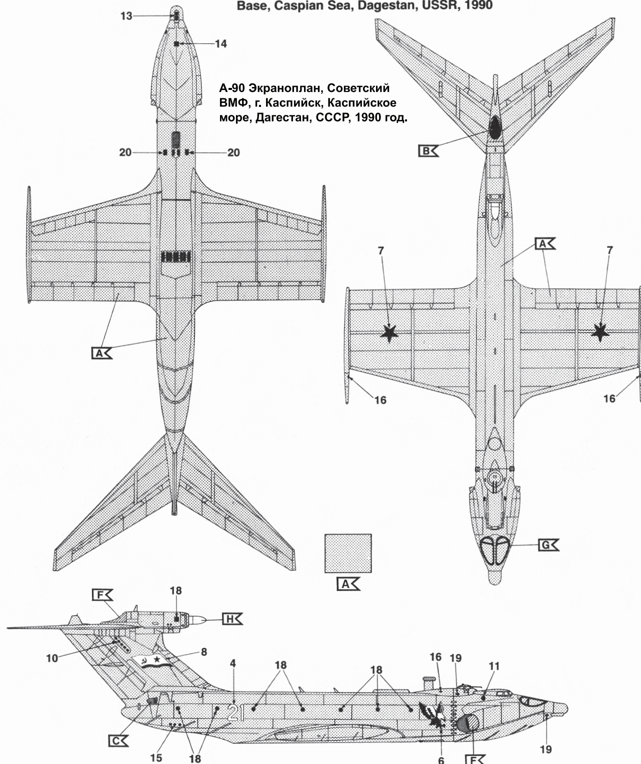
A-90 Ekranoplan, Soviet Navy, Kaspiisk Naval Base, Caspian Sea, Dagestan, USSR, 1990
