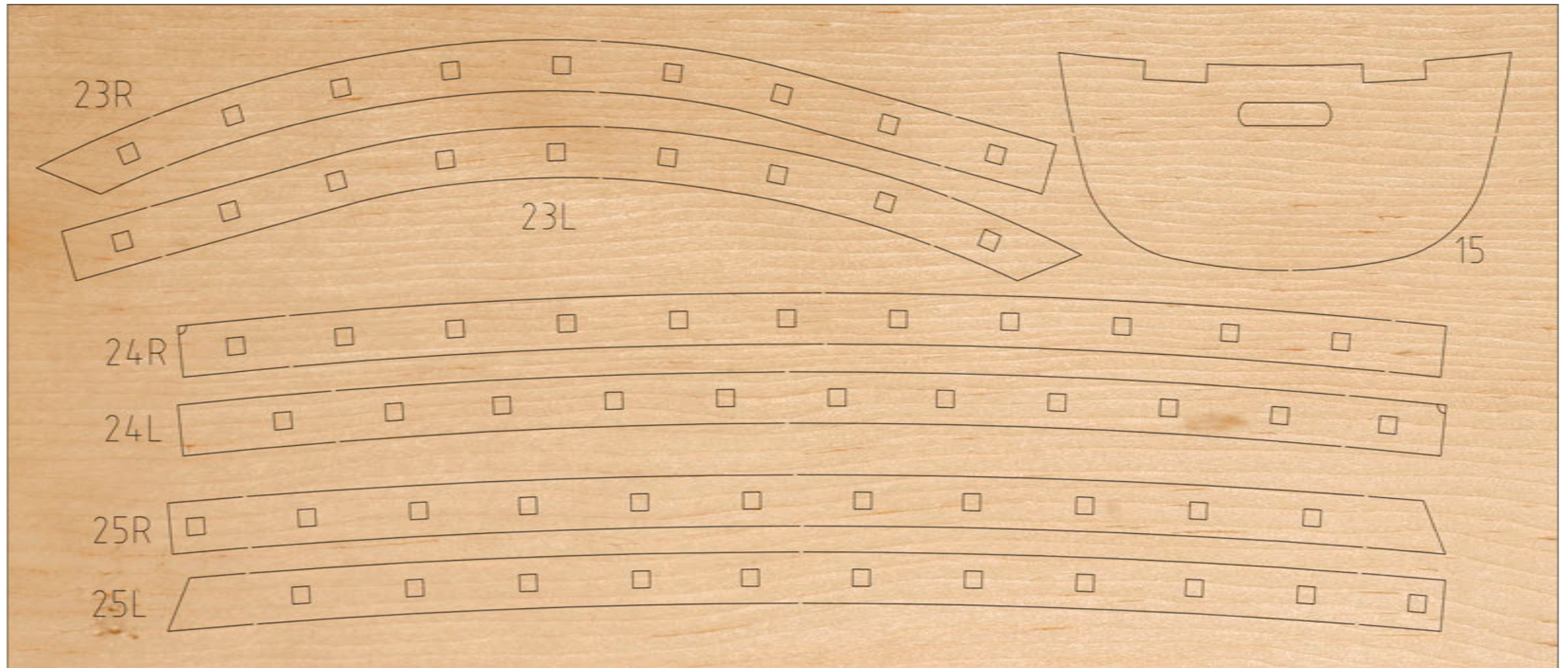
1.5mm lasercut plywood parts (180x78mm)
