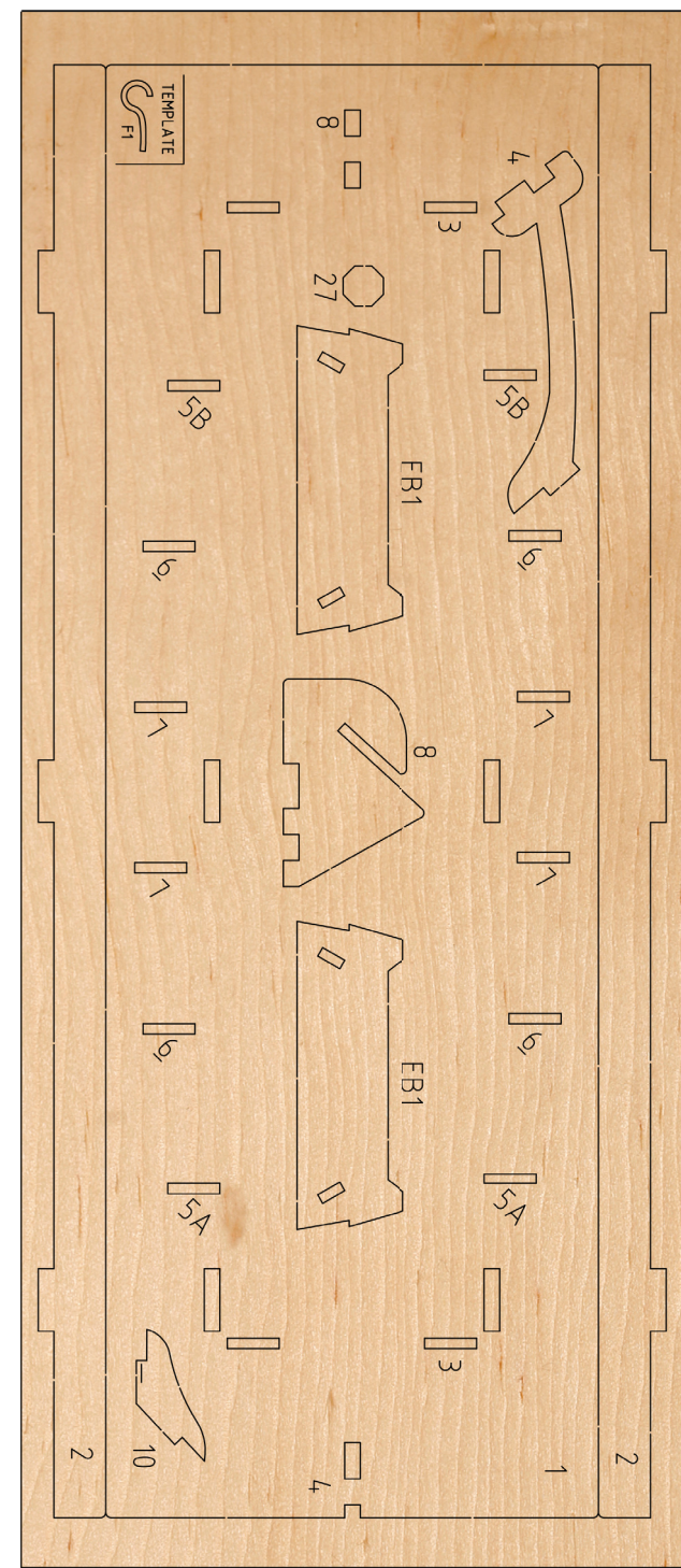
3mm plywood part 300x128mm
