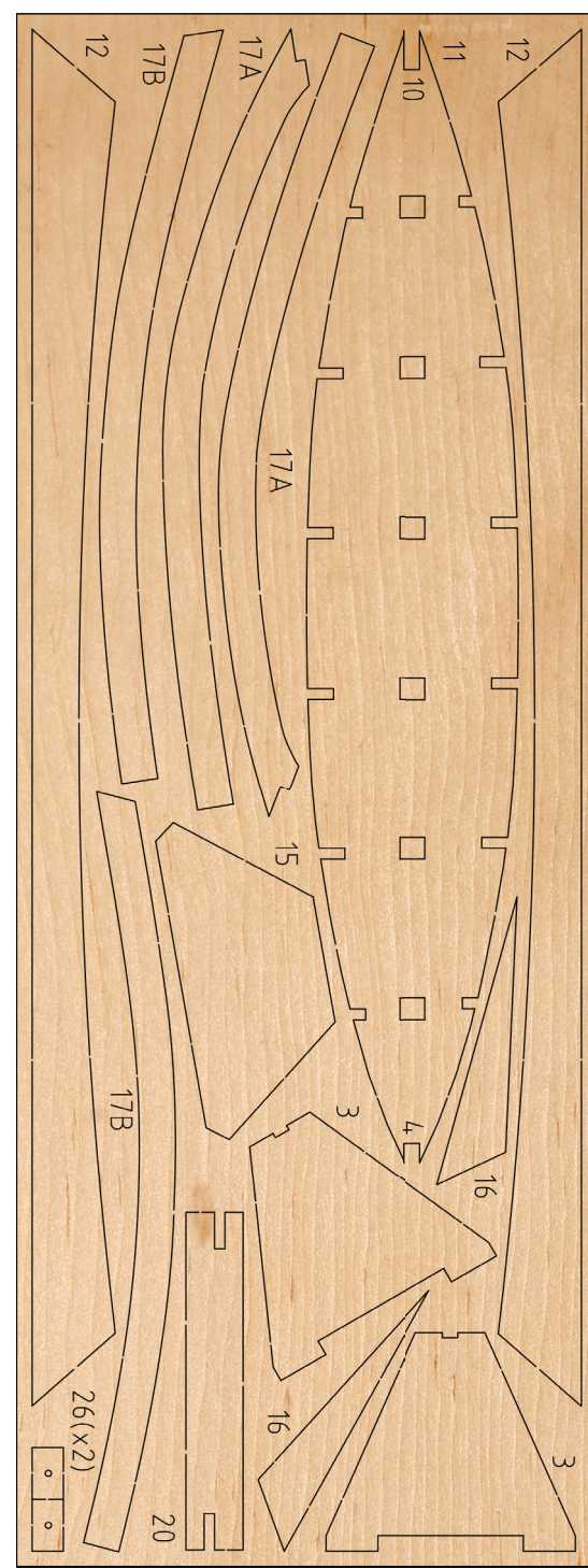
2mm plywood part 300x112mm
