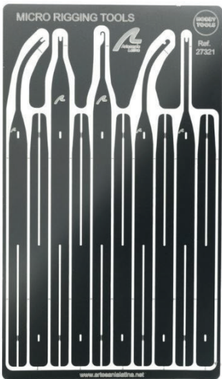
Micro Rigging Tools for Ship Model
