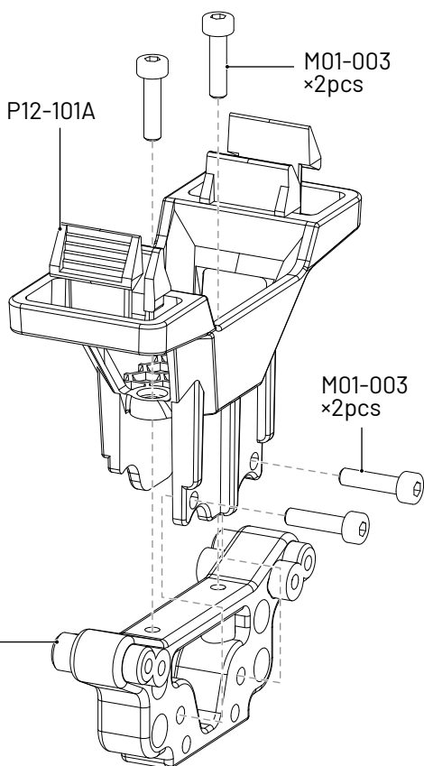
Rear lock
