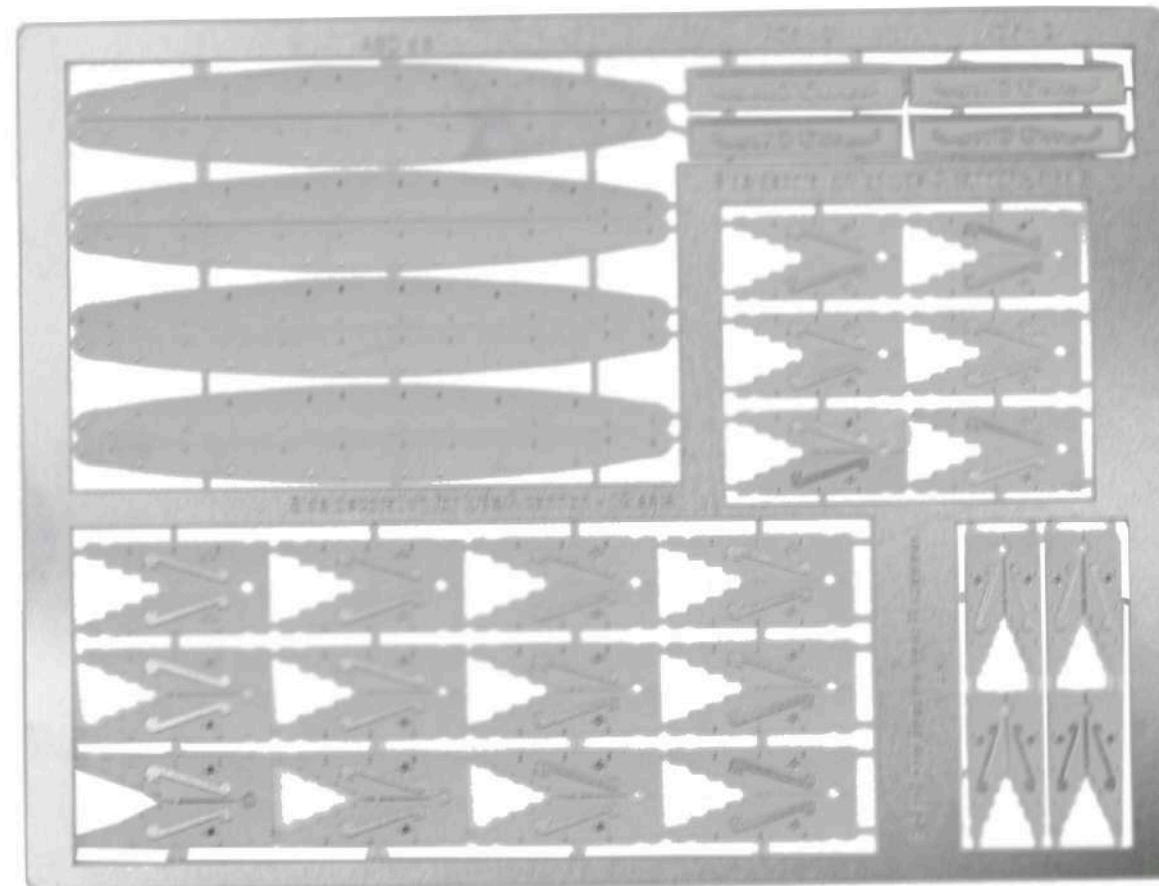
0,2mm stainless steel photoetched parts
