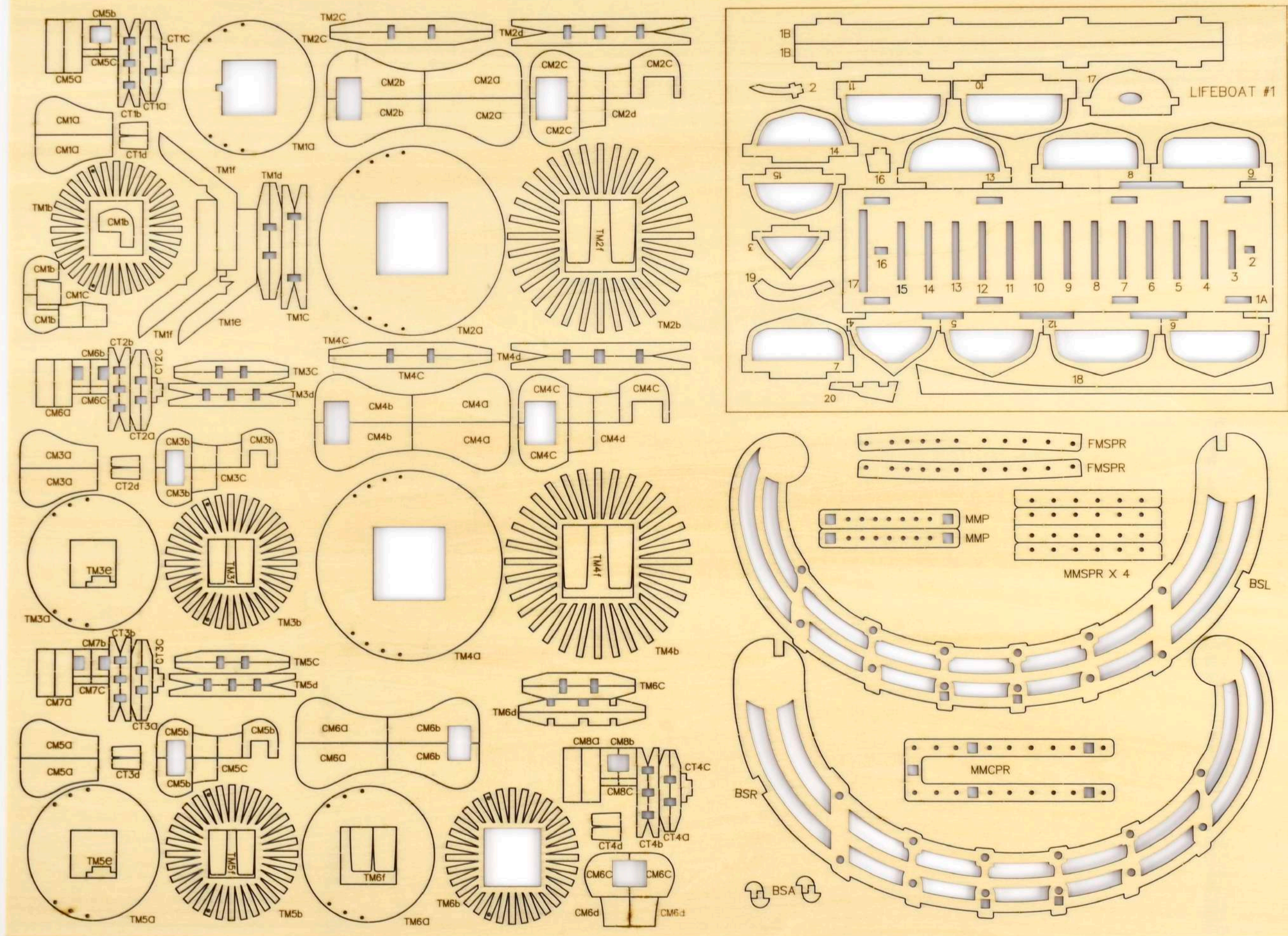
2mm lasercut plywood parts
