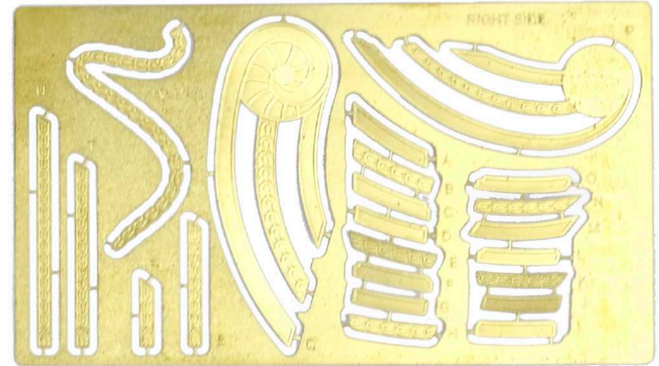
0,2mm brass photoetched parts
