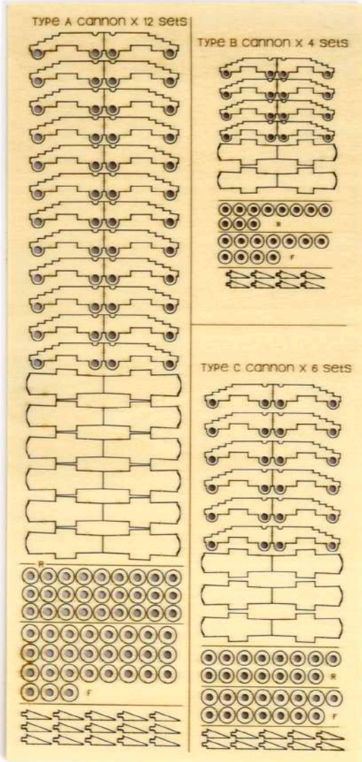
1,5mm lasercut plywood parts
