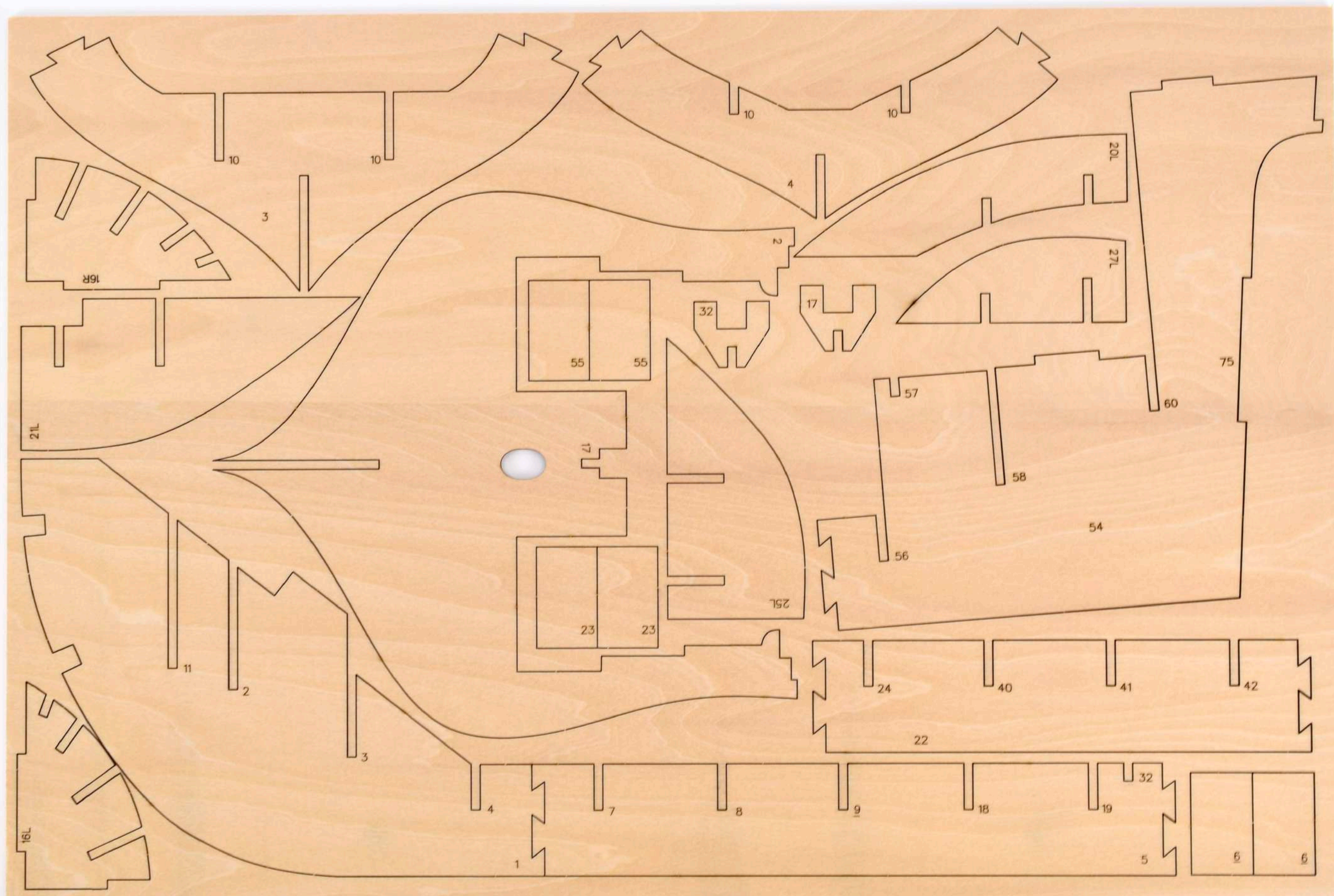
3mm lasercut plywood parts
