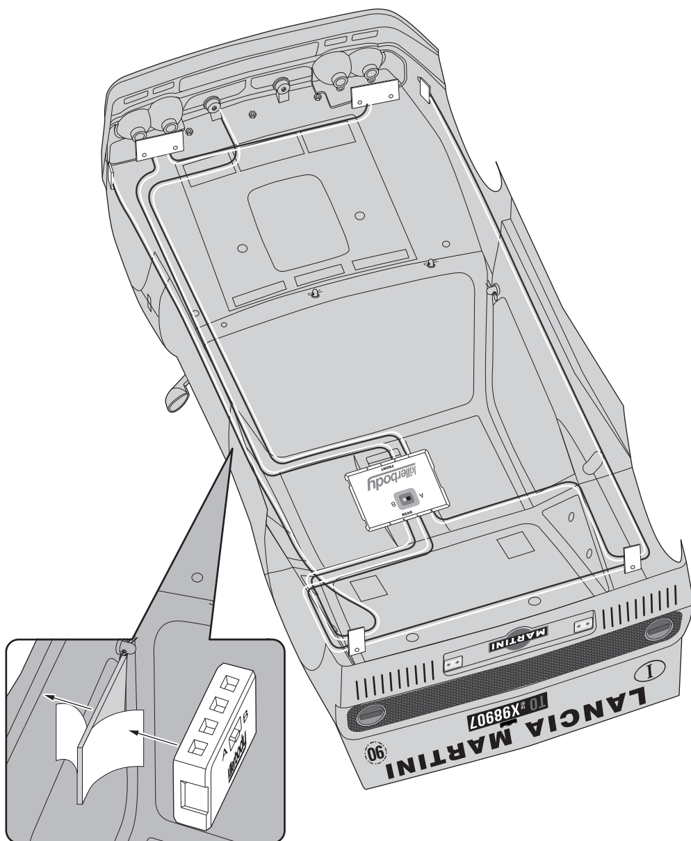
Receiver installation location
