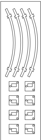
Type G carronade details x 4
