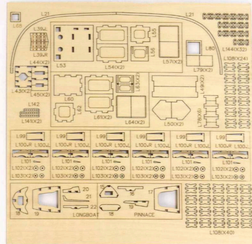
1,5mm lasercut plywood parts
