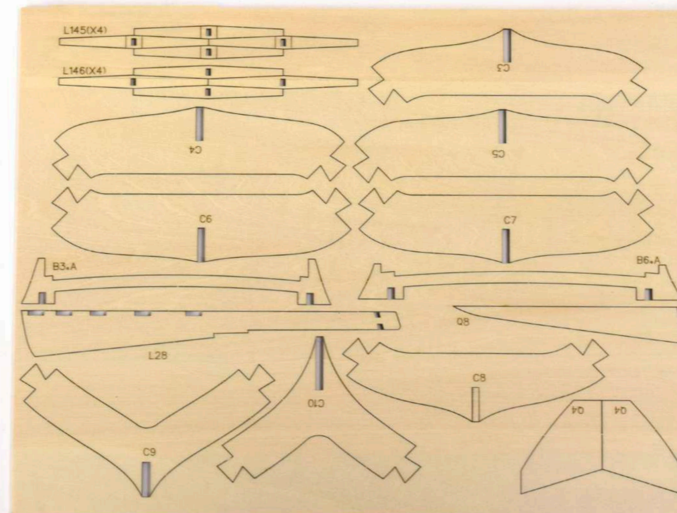
3mm lasercut plywood parts
