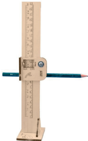
Waterline Marker for Model Ships
