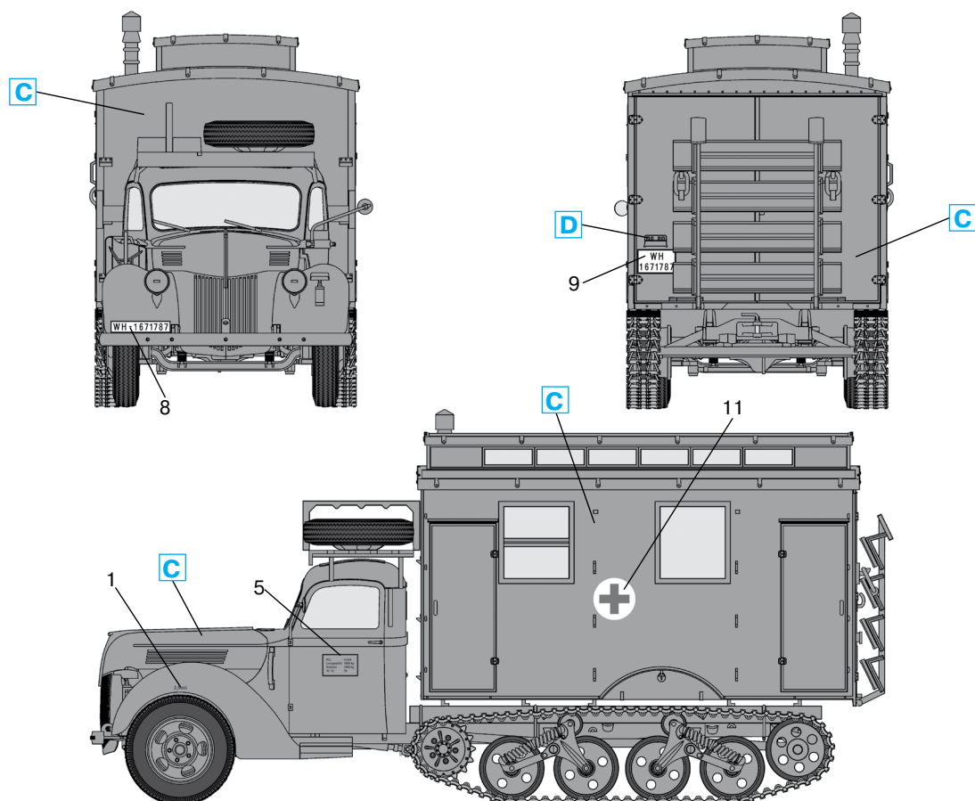
V3000S/SS M Maultier с будкой, Германия, зима 1945 г. V3000S/SS M Maultier with Shelter, Germany, Winter 1945
