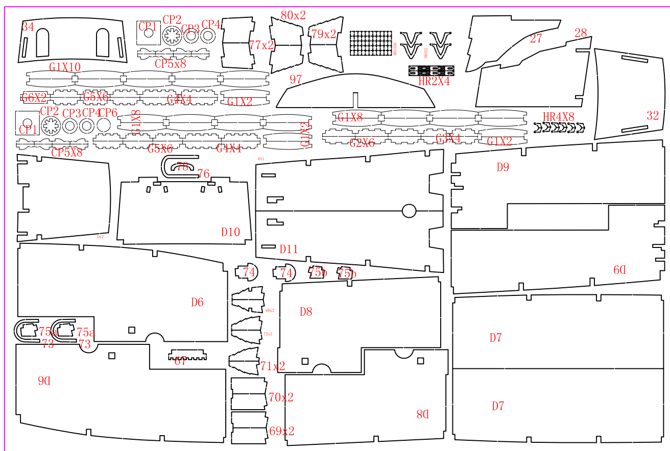
2*300*450mm plywood
