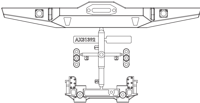
AX31392 JCR Vanguard Front Bumper Set x1
