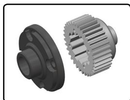
C-00250-071 Pignon de diff Métal - Couvercle de diff Composite - 34T - 1 Jeu
