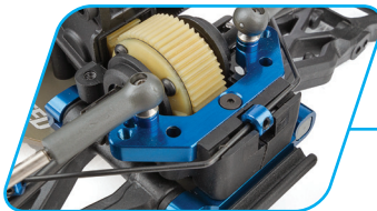
Gear Differential and Anti-Roll Bars
